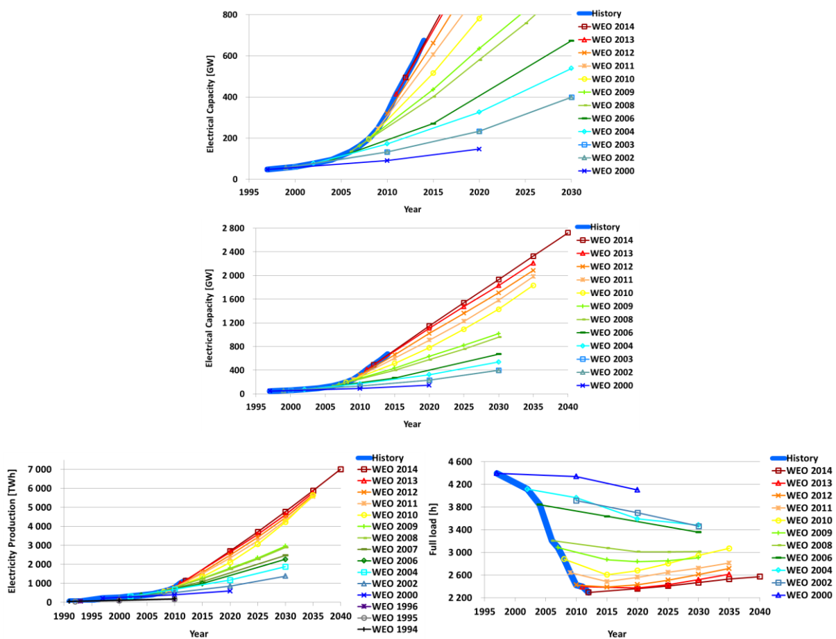
Fig. 11: New renewable capacity excluding hydro power (top and center), electricity generation (bottom, left) and renewable full load hours (bottom, right) for the years 1991 to 2040. The historical data are given for the years 1997 to 2014 for electrical capacity, from 1991 to 2012 for electricity generation and from 1997 to 2012 for full load hours. The projections range from 2010 to 2040 for both electrical capacity and full load hours and from 2000 to 2040 for generated electricity. Data are based on WEO 1994 to WEO 2014 [3-23], Werner et al. [26] and REN21 [78].
