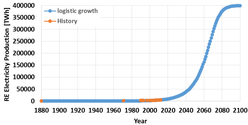
Fig. 16: Logistic growth for potential development of RE electricity production. The historic data [3-23, 75, 76] are plotted as well (orange). The parameters for the logistic growth function are according to Eq. 1: A (8 TWh), K (400000 TWh), B (0.2), v (2.7), Q (75) and M (2050).
