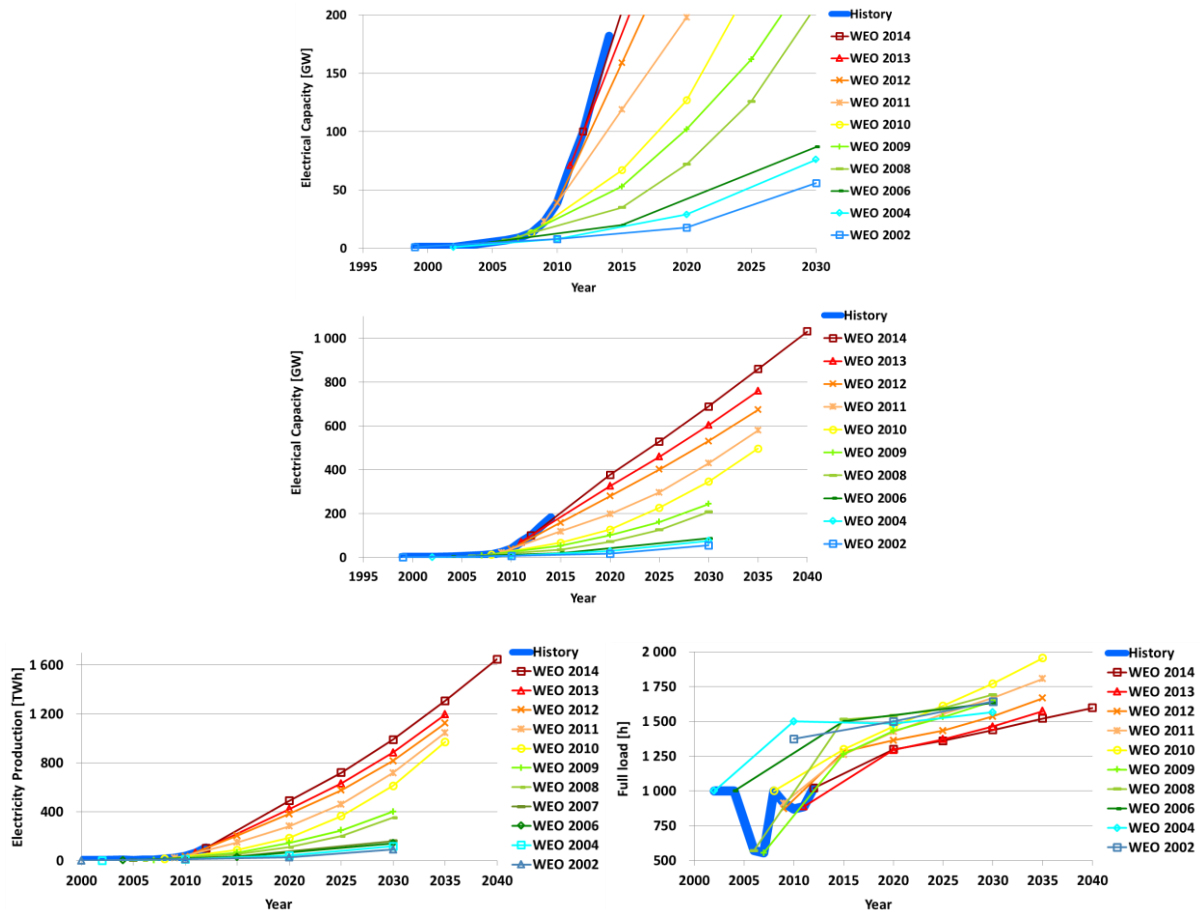
Fig. 5: Solar capacity (top and center), electricity generation (bottom, left) and solar full load hours (bottom, right) for the years 1999 to 2040. The historical data are given for the years 1999 to 2014 for electrical capacity, from 2000 to 2012 for electricity generation and from 2002 to 2012 for the full load hours. The projections range from 2010 to 2040. Data are based on WEO 2002 to WEO 2014 [13-23], Werner et al. [26] and REN21 [78].
