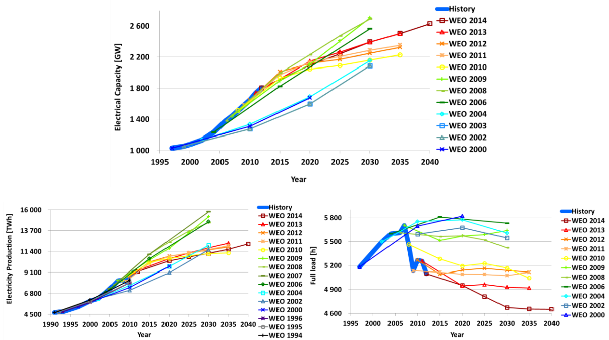
Fig. 12: Coal power (top), electricity generation (bottom, left) and coal full load hours (bottom, right) for the years 1991 to 2040. The historical data are given for the years 1997 to 2012 for both electrical capacity and full load hours and from 1991 to 2012 for electricity production. The projections range from 2010 to 2040 for both electrical capacity and full load hours and from 2000 to 2040 for generated electricity. Data are based on WEO 1994 to WEO 2014 [3-23].
